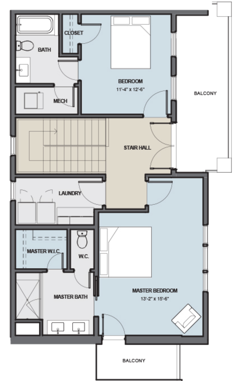
UNIT 12 - SECOND FLOOR PLAN
