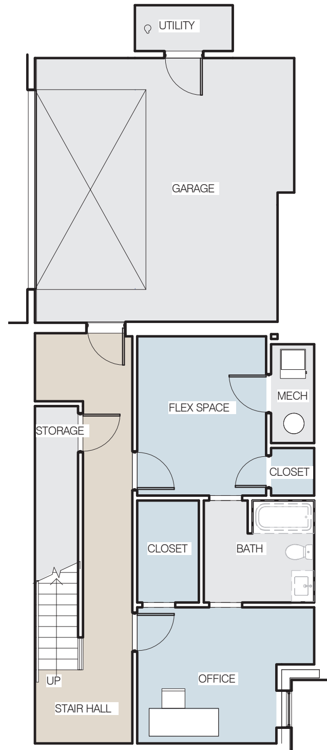
1 BASEMENT FLOOR PLAN SCALE: 1/8" = 1'-0"
