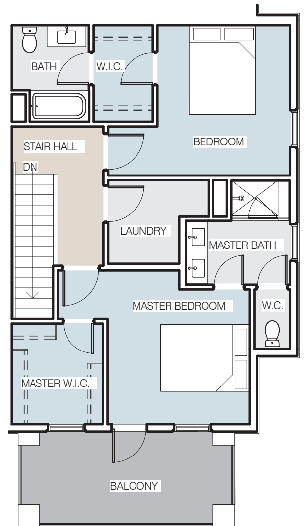
3 SECOND FLOOR PLAN SCALE: 1/8" = 1'-0"
