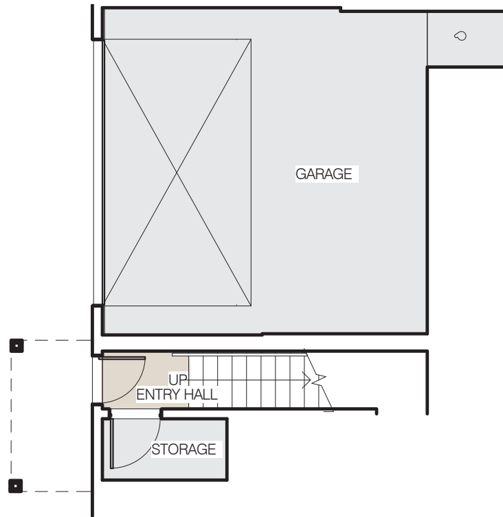
1 BASEMENT FLOOR PLAN SCALE: 1/8" = 1'-0"
